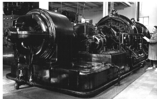
SAQ alternator (photo credit: Tekniska museet).
