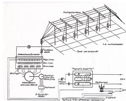
SAQ circuit diagram (17.2 kHz, 200 kW).
